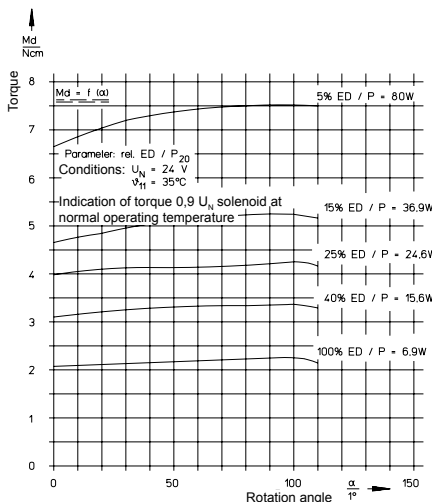
Fig. 6: Characteristics M_d = f(\alpha) Type G DR X 035 MSM-Fo 0804.1692
