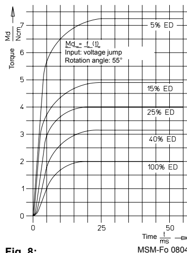
Fig. 8: Characteristics M_d = f(t) Type G DR X 035 MSM-Fo 0804.1675
