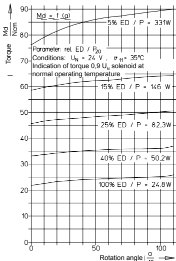
Fig. 12: Characteristics M_d = f(\alpha) Type G DR X 075 MSM-Fo 0804.1694
