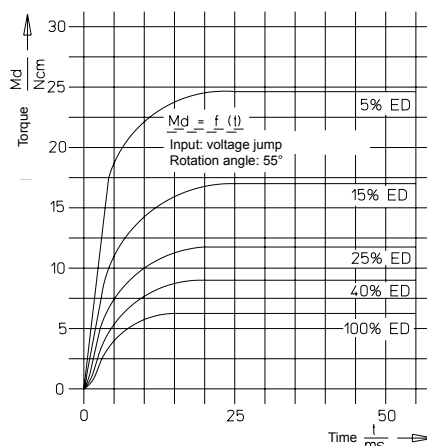
Fig. 11: Characteristics M_d = f(t) Type G DR X 050 MSM-Fo 0804.1676
