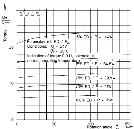
Fig. 9: Characteristics M_d = f(\alpha) Type G DR X 050 MSM-Fo 0804.1693
