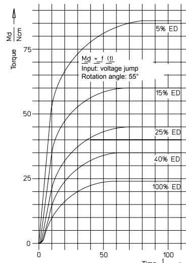
Fig. 14: Characteristics M_d = f(t) Type G DR X 075 MSM-Fo 0804.1677
