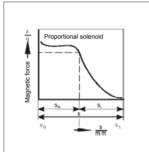
Fig. 3: Force vs. stroke characteristic
