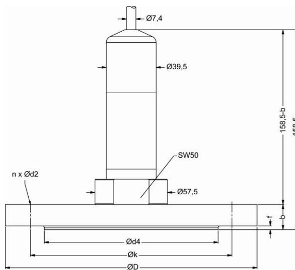
flange version
