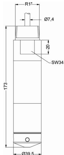
thread R1" for stainless steel pipe
