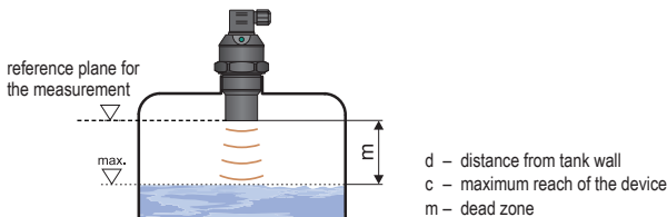
Fig. 2: Dead zone of the device
