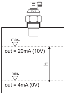
Fig. 33: Default mode (level measurement)
