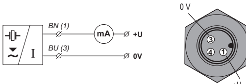
Fig. 22: Connection diagram of the ULM level meter (variant -I) and view of the connector
