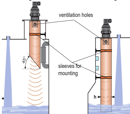
Fig. 6: Short guide tube installation
