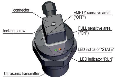
Fig. 32: Key parts of the measuring device (version with Hall probes)
