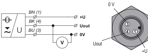
Fig. 23: Connection diagram of the ULM level meter (variant -U) and view of the connector
