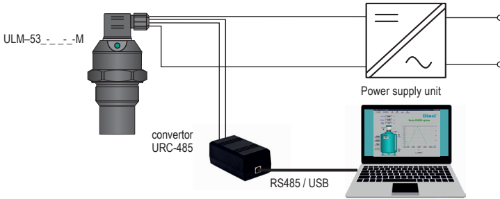
Obr. 35: Typical hardware configuration with Modbus®
