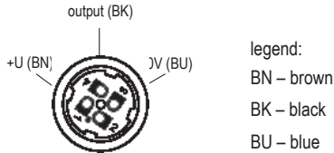
Fig. 21: Inside view of the connector socket
