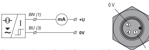
Fig. 24: Connection diagram of the ULS sensor with S type output (two-state current switch 4 mA / 20 mA)
