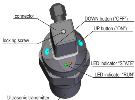
Fig. 31: Key parts of the measuring device (version with buttons)
