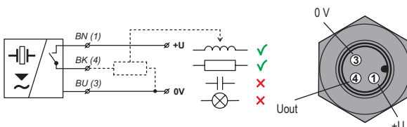
Fig. 25: Connection diagram of the ULS sensor with P type output (PNP) with an open collector
