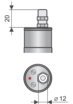
Variants "D" with cable outlets
