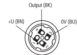
Inside of the connector socket (Variant "C")
