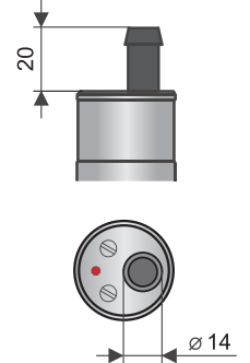
Variants "B" with cable outlets
