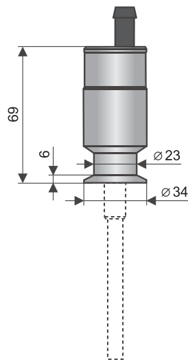
Variants "C" with connector
