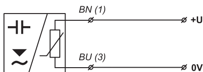
NAMUR type sensors connection (version Xi; XiT; XiM; XiMT)
