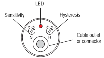
Top view of level sensor
