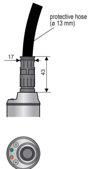
Design "H" with cable gland for protected hoses – for using in an outdoor environment or in an area with increased moisture.
