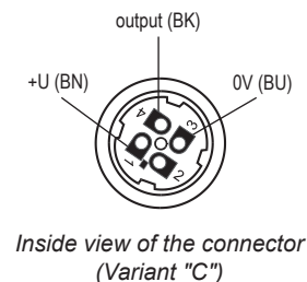
PNP output type sensor connection
