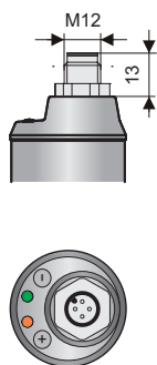
Design "C" with connector M12
