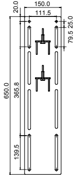
(A) Base Plate
